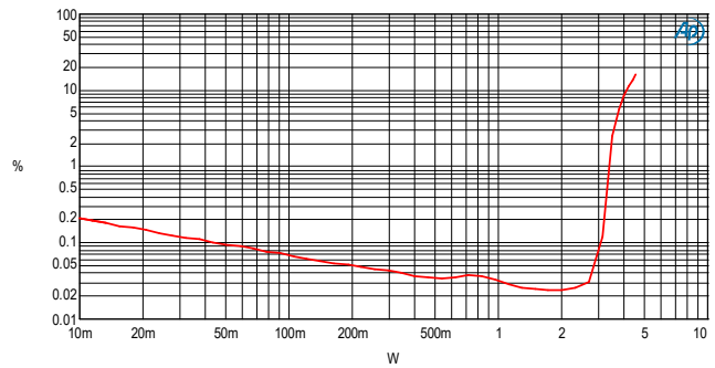
Po vs THD+N.ats2
