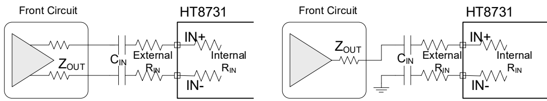
Figure 2 (1) Differential Input;
